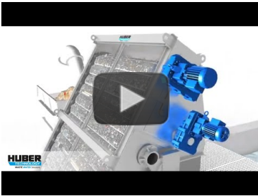
Animation: HUBER Lochblech-Umlaufrechen EscaMax® https://www.youtube.com/watch?v=pr_o1Eu57cg
