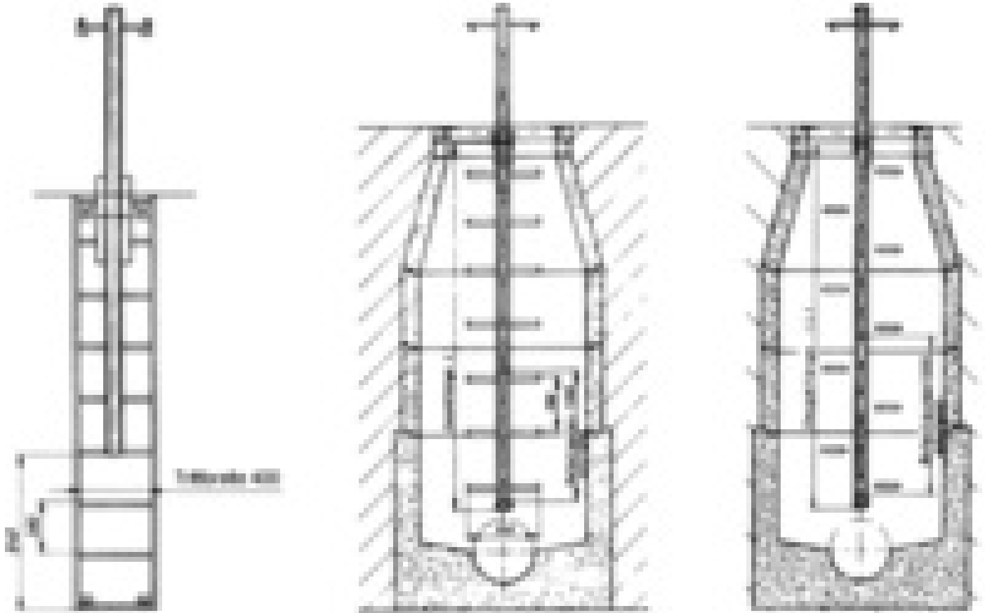
HUBER safety climbing systems - with safety ladder SiS2, as climbing device SiS3, with step irons SiS4
